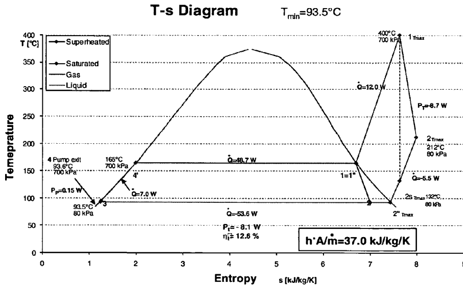
(b) T-s diagram for a condenser temp. T_{\text{min}}=93.5^\circ\text{C} , defined for in-cabin or ground operation
