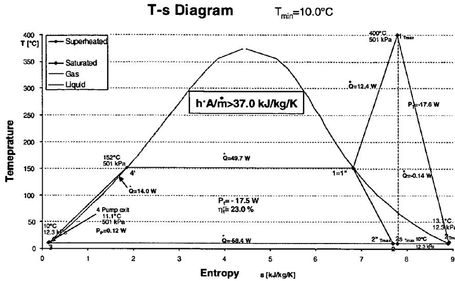
(a) T-s diagram for a condenser temperature of T_{\text{min}}=10^\circ\text{C} , defined for in-flight operation
